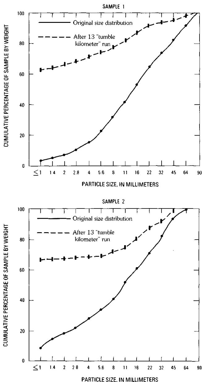
FIGURE 12.—Cumulative particle-size distribution curves for samples used in attrition experiment. Note that in both cases nearly two-thirds of the material broke down to the less-than-2-mm fraction after 13 "tumble kilometers." The tumbling experiment involved a Los Angeles Rattler Machine, which was used to determine attrition rates on dry sediment samples.
