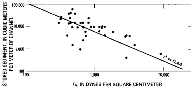
FIGURE 20.—Logarithmic plot of volume of stored sediment per unit distance ( V_s ) versus the boundary shear stress ( T_b ) calculated for Redwood Creek at bankfull discharge.
