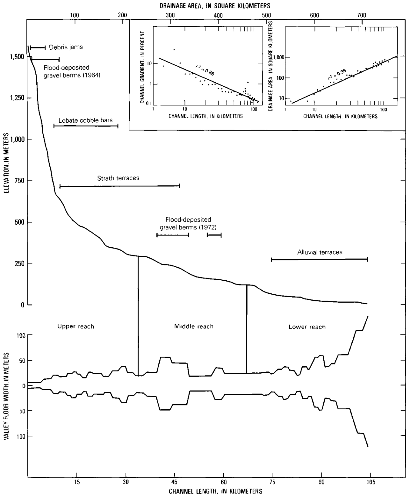
FIGURE 14.—Longitudinal profile of Redwood Creek showing distribution of localized features along certain reaches of the creek. Valley widths for Redwood Creek are drawn on the channel gradient and same horizontal scale as the profile. Strong relationships exist between channel length and between drainage area and channel length ( r^2=0.86 and 0.98 , respectively).
